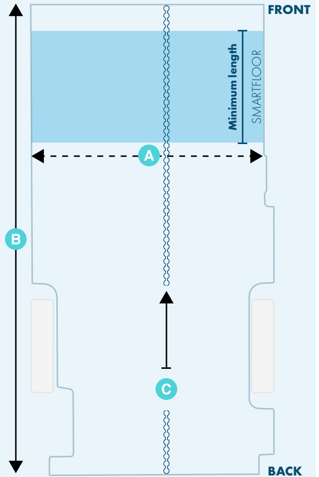
Top-view vehicle floor with minimum length of the Smartfloor
